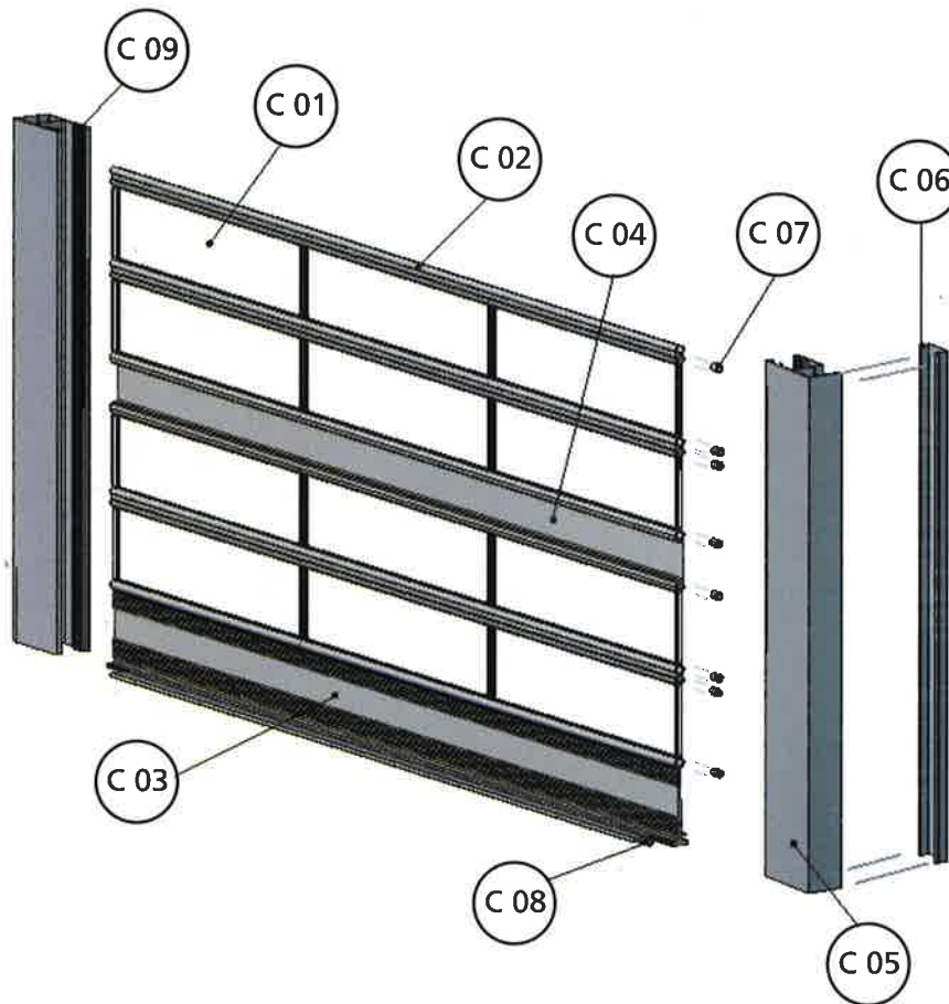
Sample Calculation of Materials Required for door W 3.0m x Ht 2.4m
